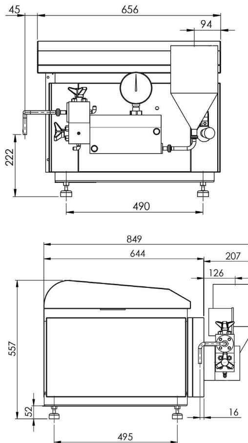
Overall dimensions (mm)
